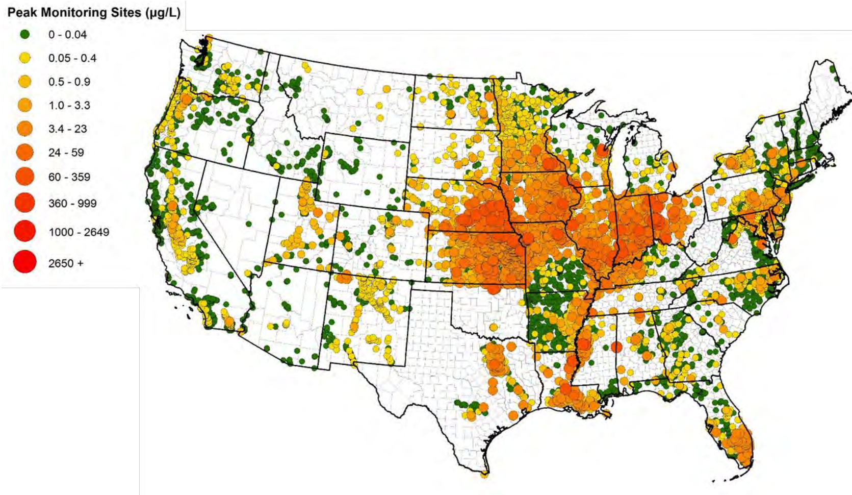
Figure 17. Distribution of the peak concentrations of atrazine for georeferenced monitoring sites.
